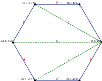
6-sided Polygon with Minimal Diagonals
